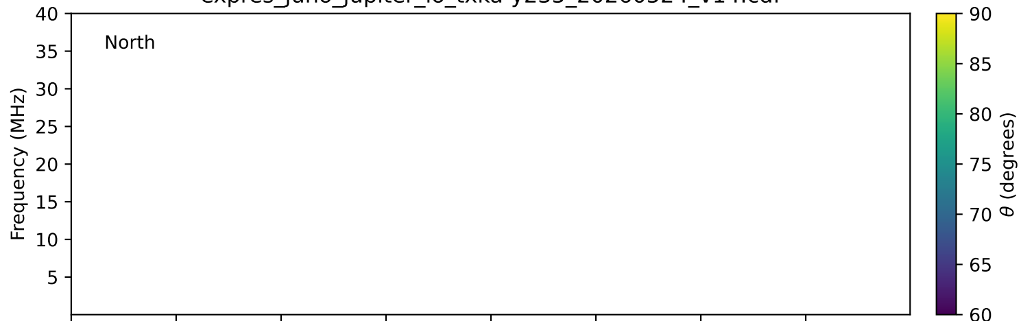
expres_juno_jupiter_io_txka-y235_20260524_v14.cdf
