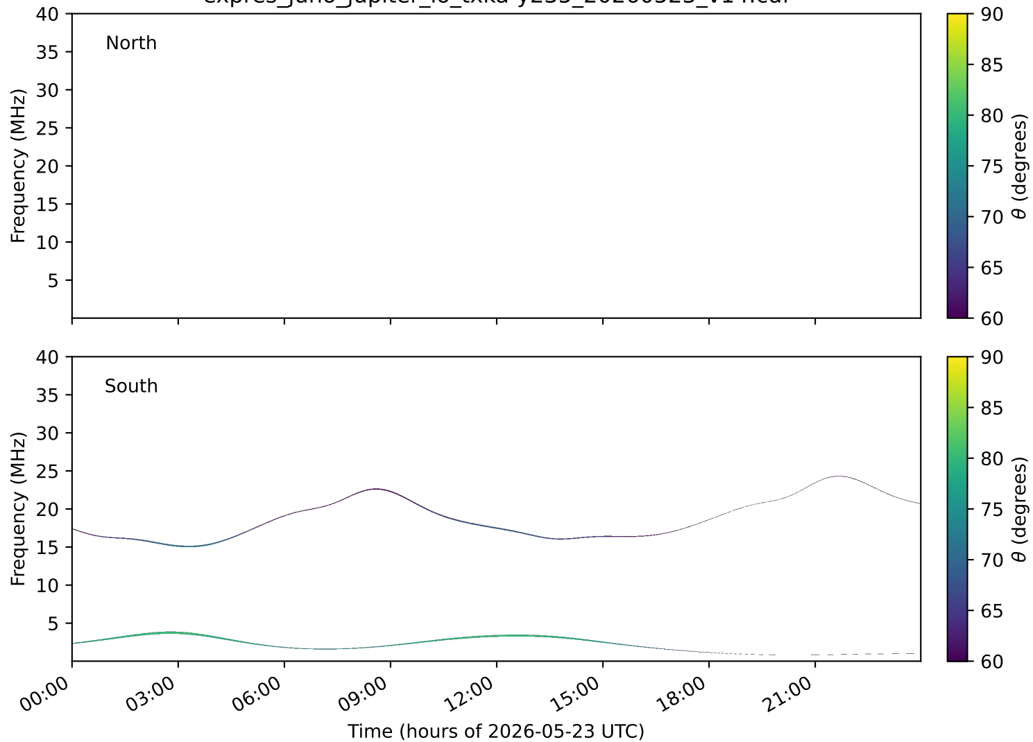
expres_juno_jupiter_io_txka-y235_20260523_v14.cdf
