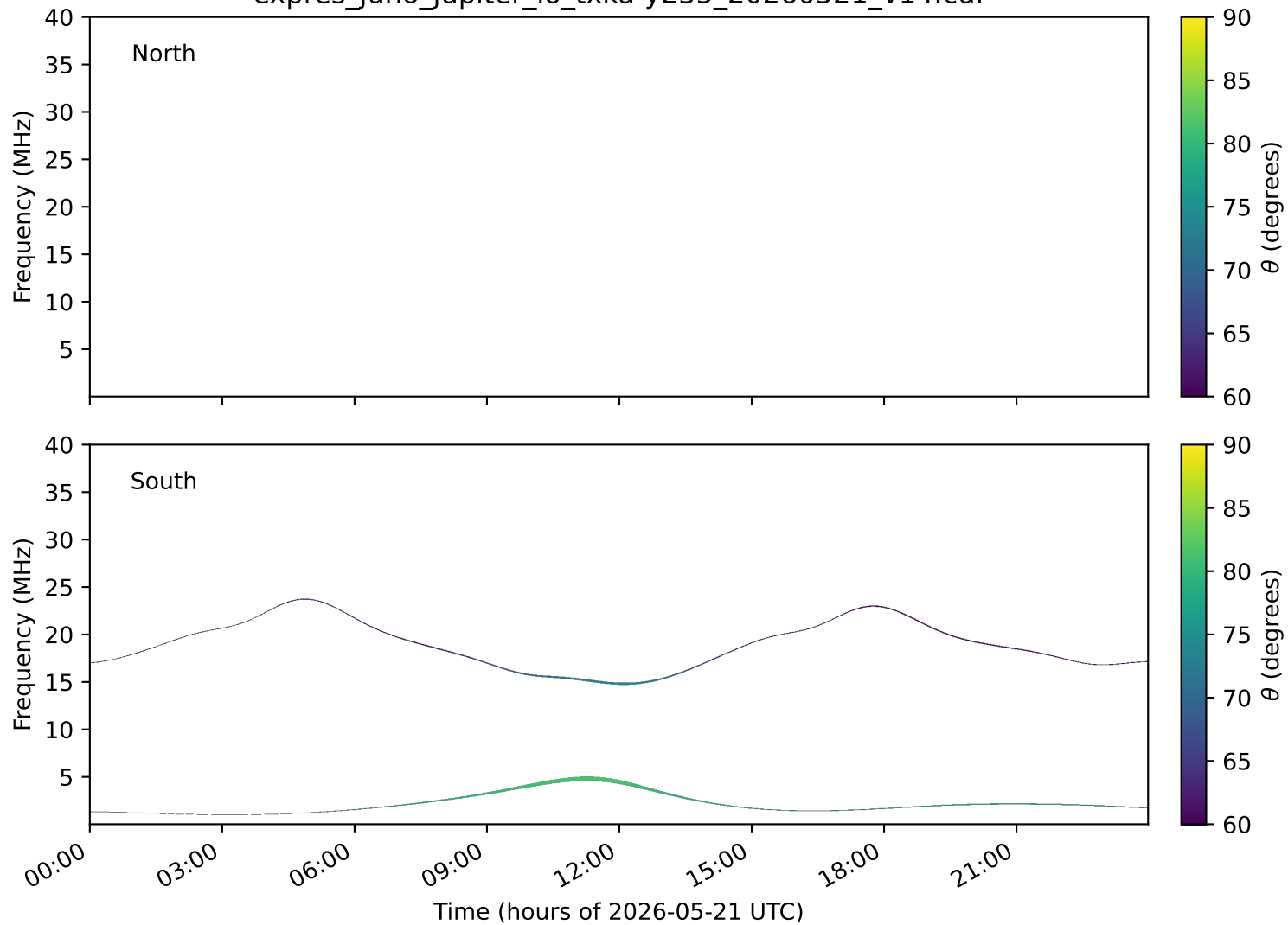
expres_juno_jupiter_io_txka-y235_20260521_v14.cdf
