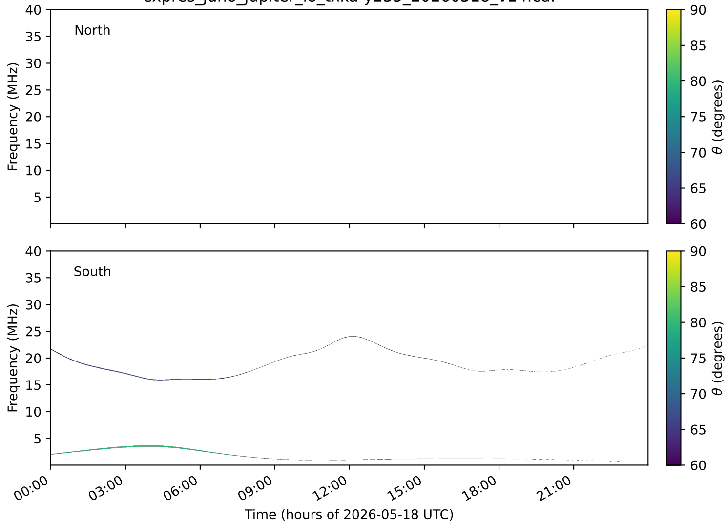
expres_juno_jupiter_io_txka-y235_20260518_v14.cdf
