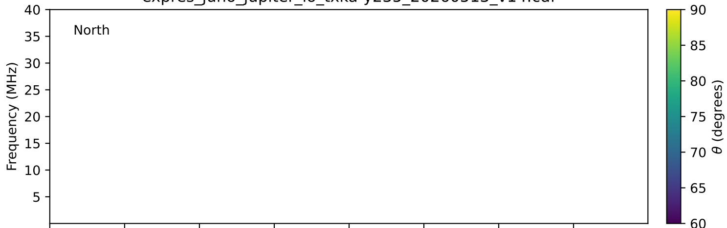
expres_juno_jupiter_io_txka-y235_20260513_v14.cdf
