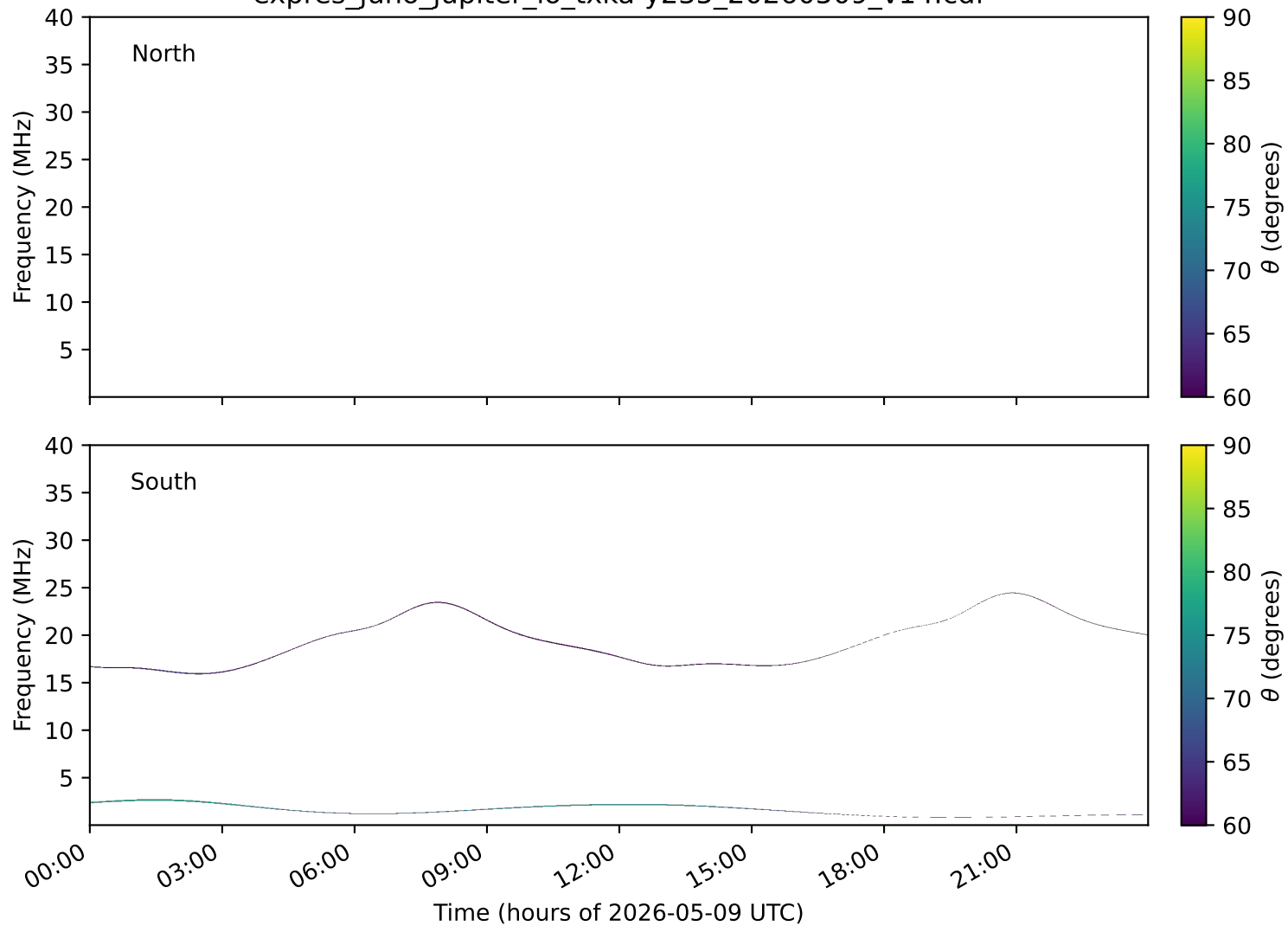
expres_juno_jupiter_io_txka-y235_20260509_v14.cdf
