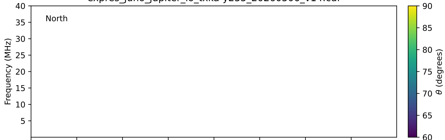
expres_juno_jupiter_io_txka-y235_20260506_v14.cdf
