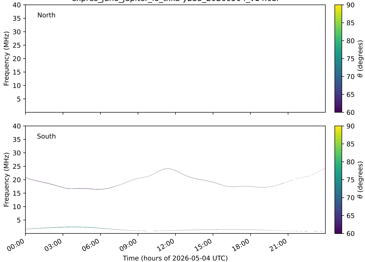
expres_juno_jupiter_io_txka-y235_20260504_v14.cdf
