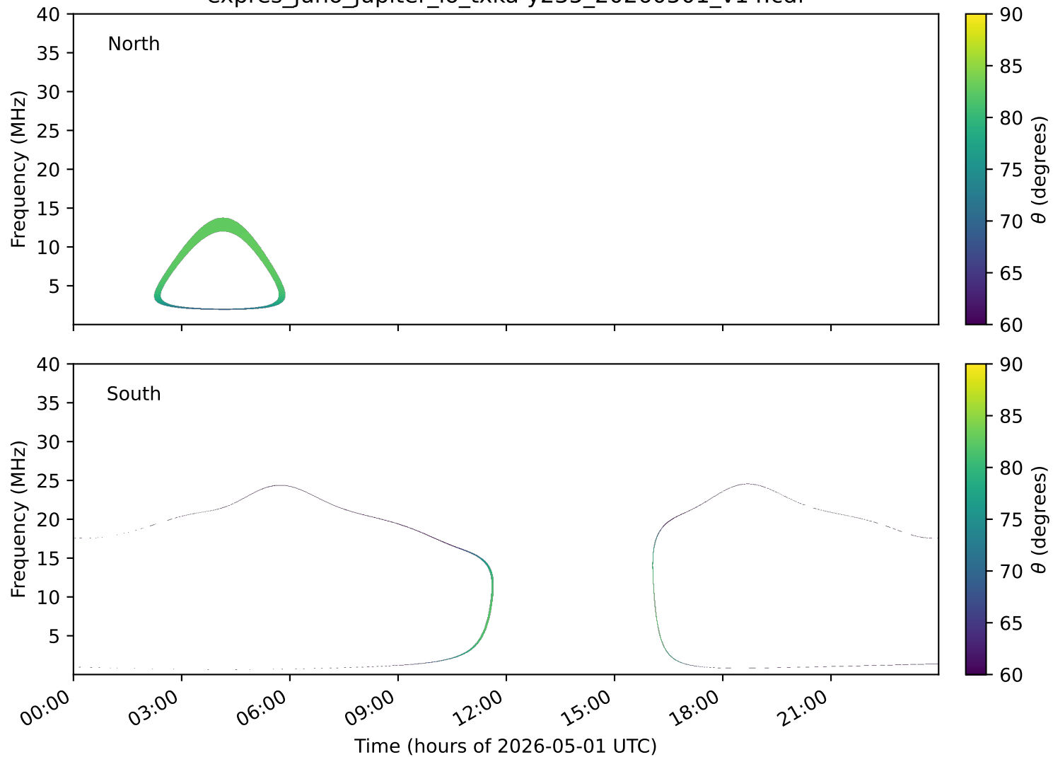
expres_juno_jupiter_io_txka-y235_20260501_v14.cdf
