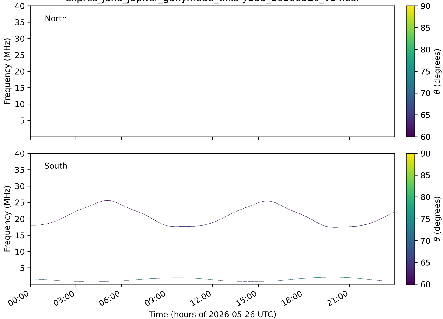
expres_juno_jupiter_ganymede_txka-y235_20260526_v14.cdf
