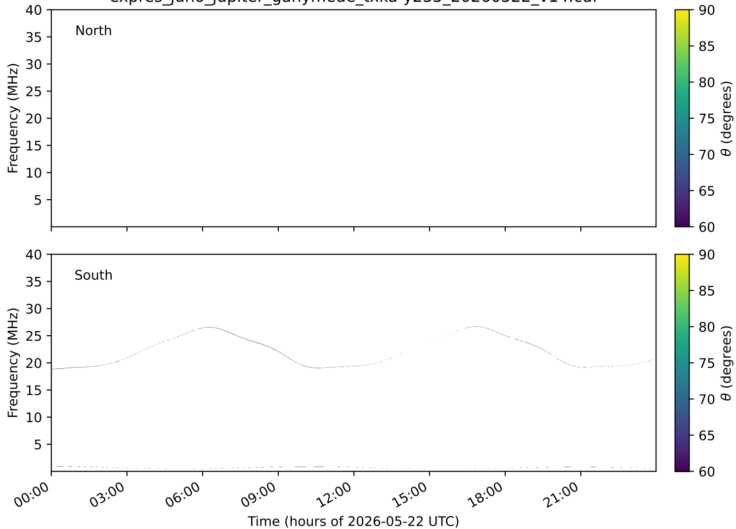
expres_juno_jupiter_ganymede_txka-y235_20260522_v14.cdf
