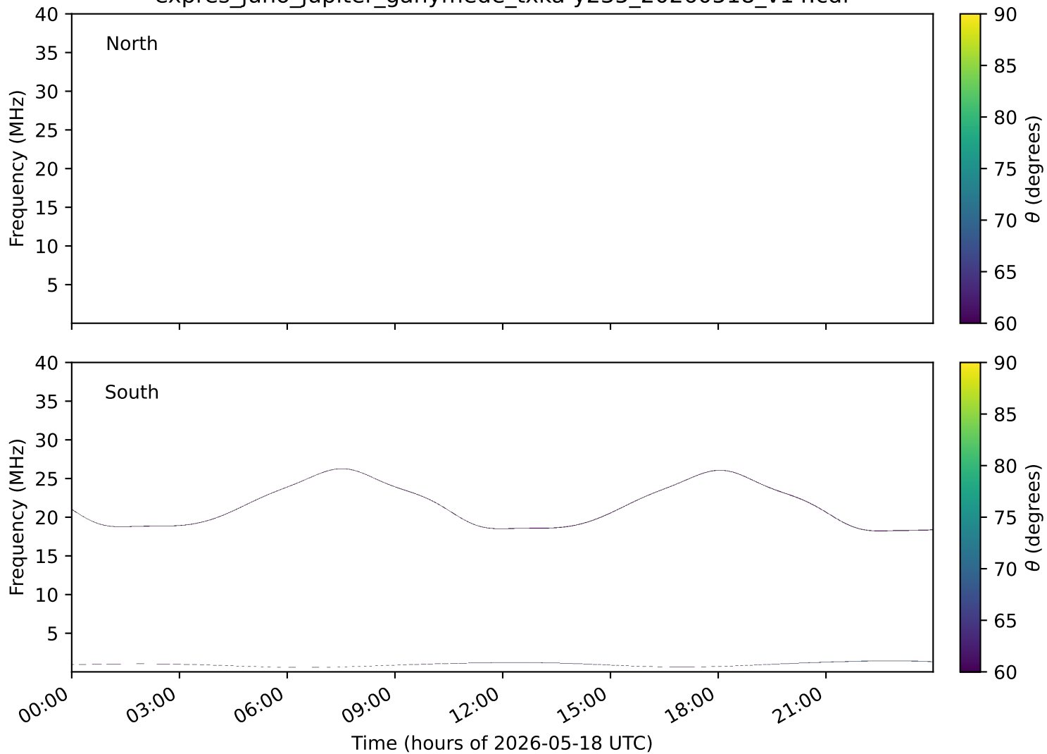
expres_juno_jupiter_ganymede_txka-y235_20260518_v14.cdf
