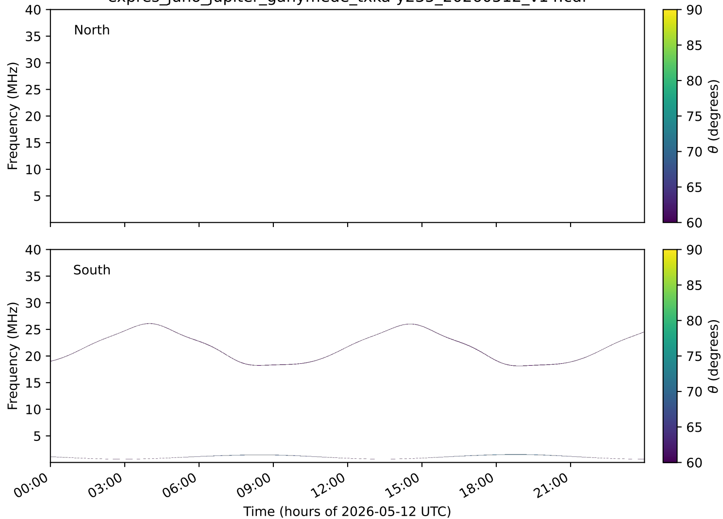
expres_juno_jupiter_ganymede_txka-y235_20260512_v14.cdf
