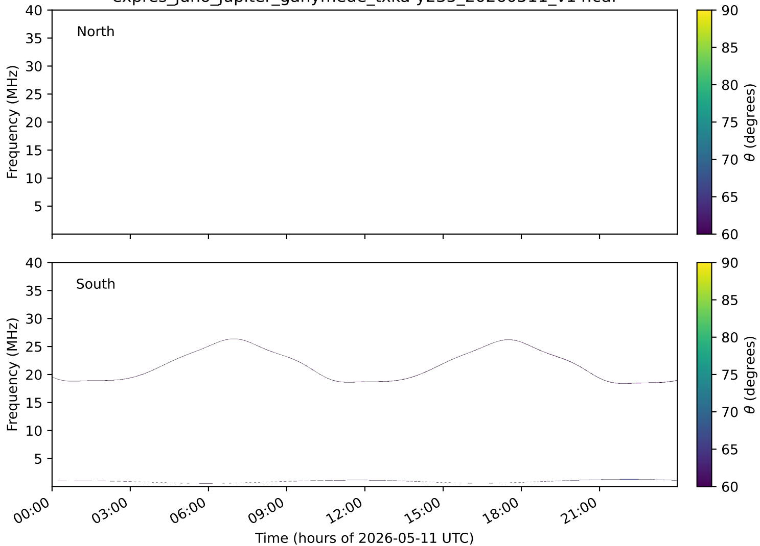
expres_juno_jupiter_ganymede_txka-y235_20260511_v14.cdf
