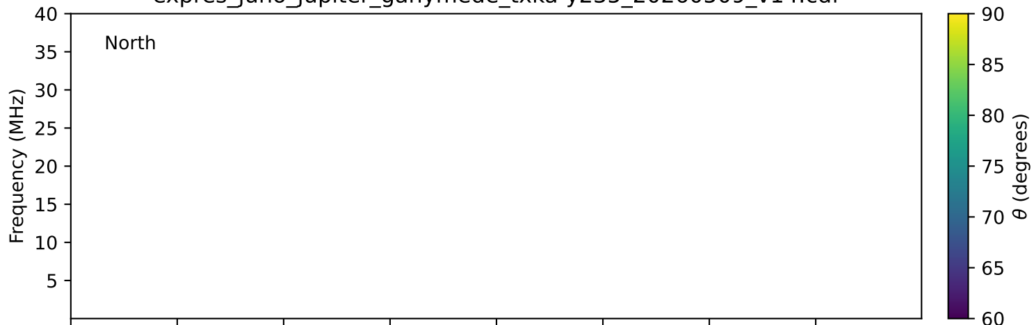
expres_juno_jupiter_ganymede_txka-y235_20260509_v14.cdf
