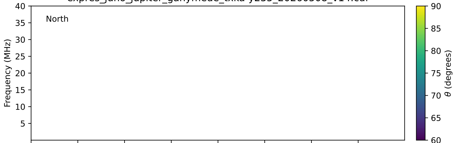
expres_juno_jupiter_ganymede_txka-y235_20260508_v14.cdf
