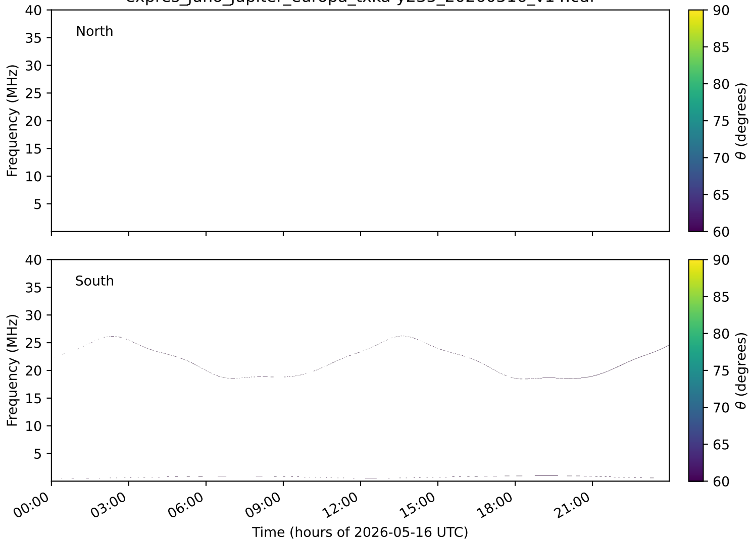
expres_juno_jupiter_europa_txka-y235_20260516_v14.cdf
