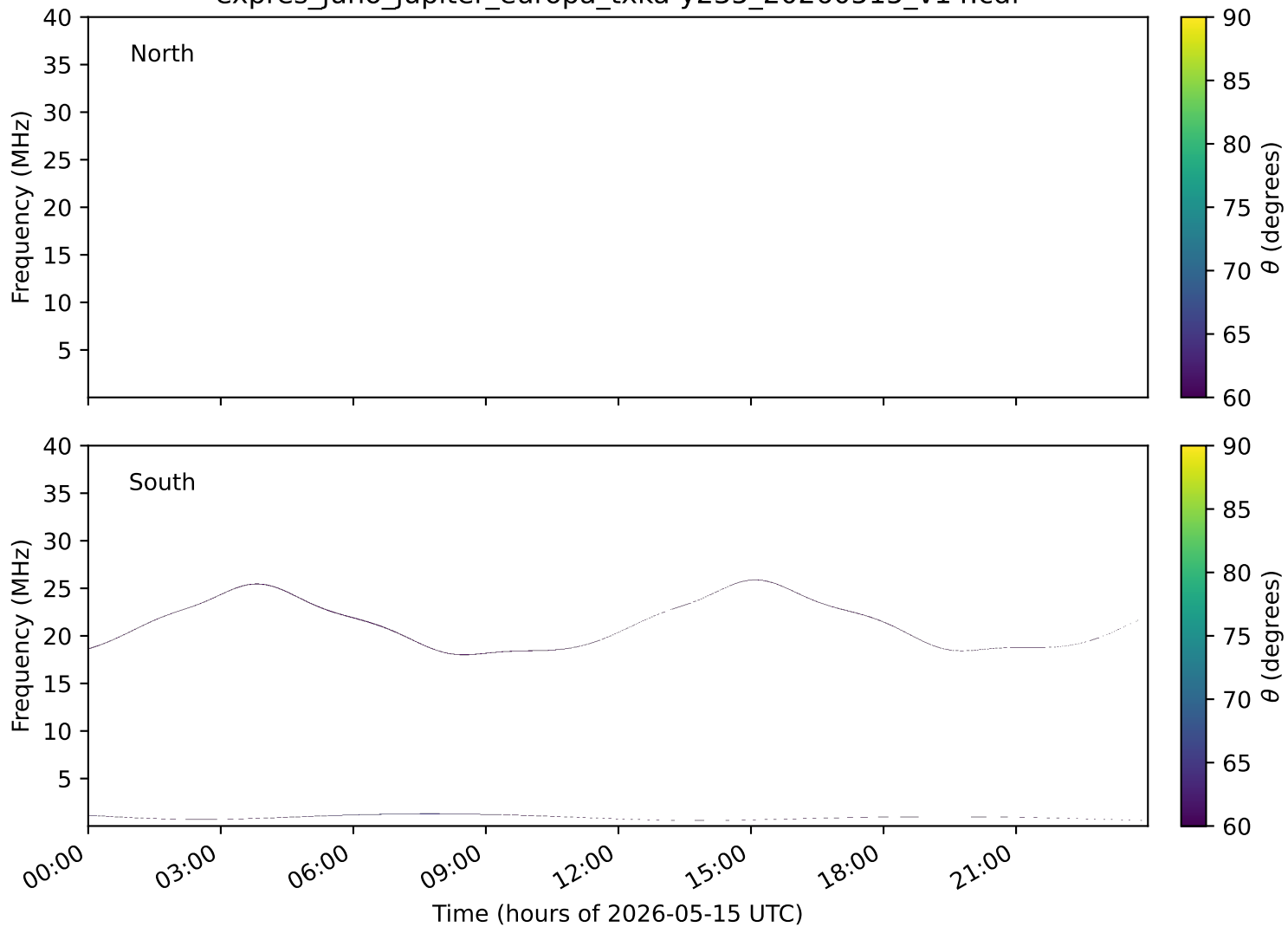
expres_juno_jupiter_europa_txka-y235_20260515_v14.cdf
