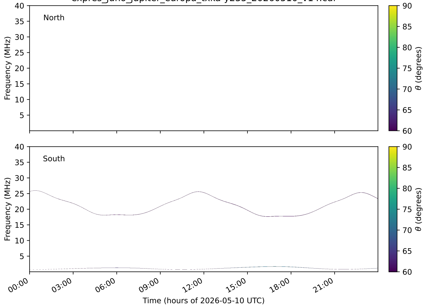
expres_juno_jupiter_europa_txka-y235_20260510_v14.cdf
