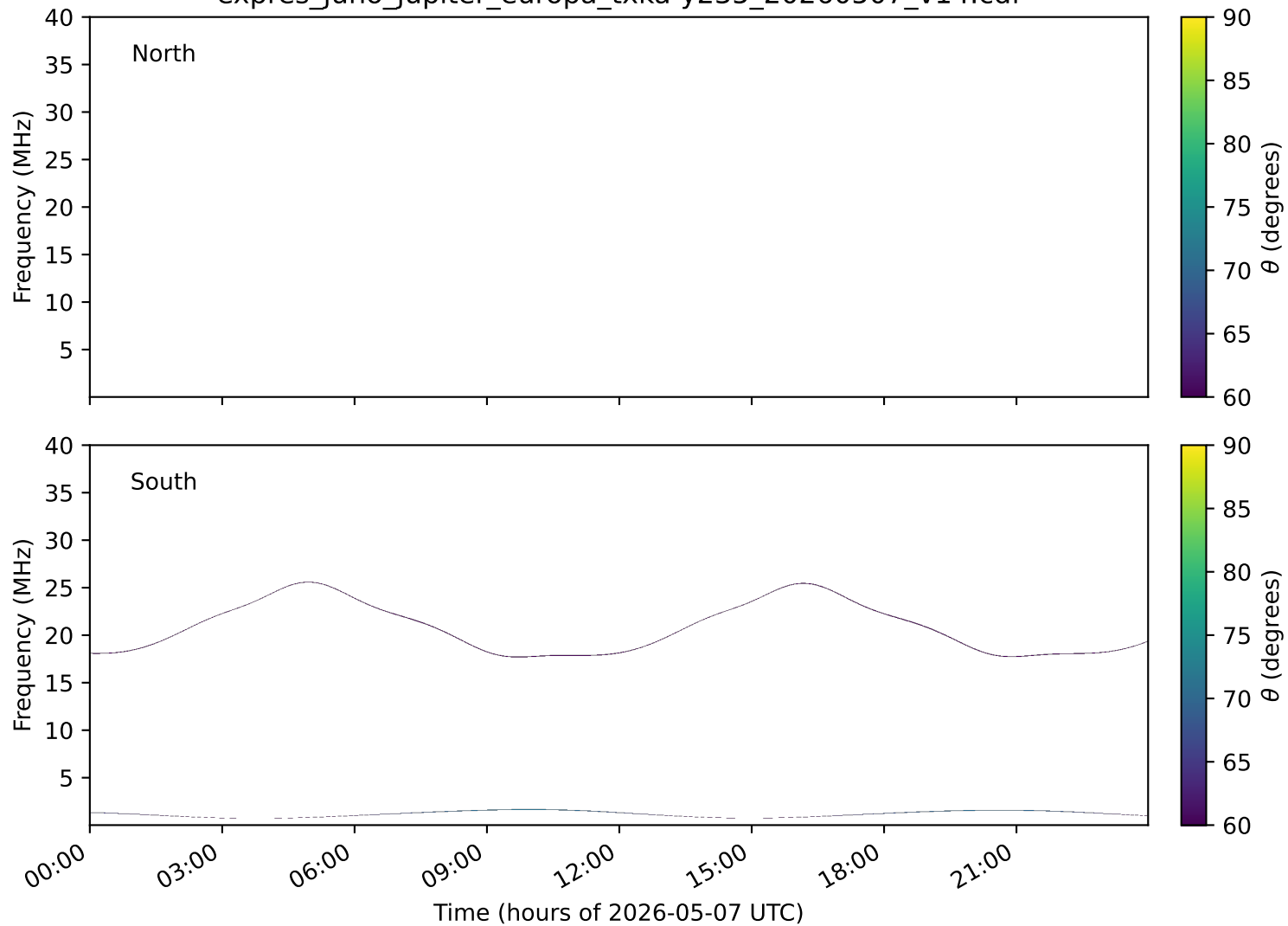
expres_juno_jupiter_europa_txka-y235_20260507_v14.cdf
