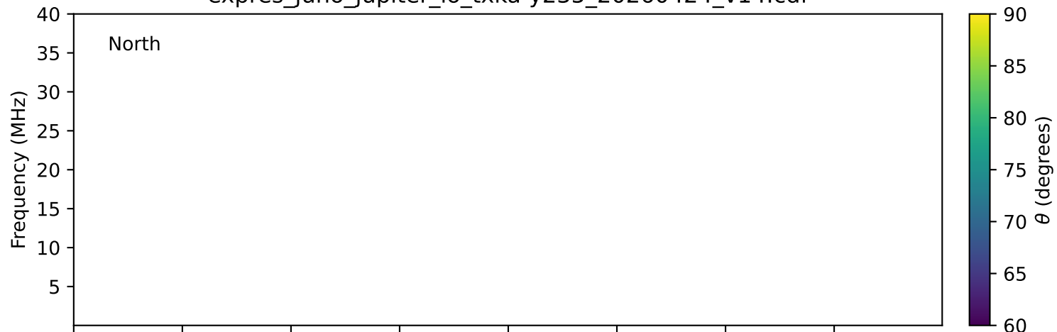
expres_juno_jupiter_io_txka-y235_20260424_v14.cdf
