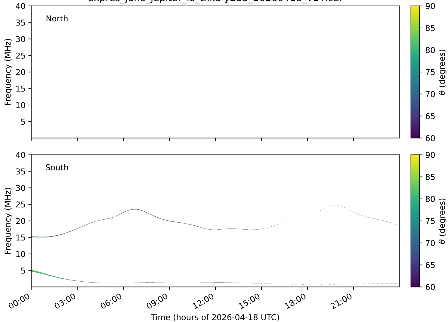
expres_juno_jupiter_io_txka-y235_20260418_v14.cdf
