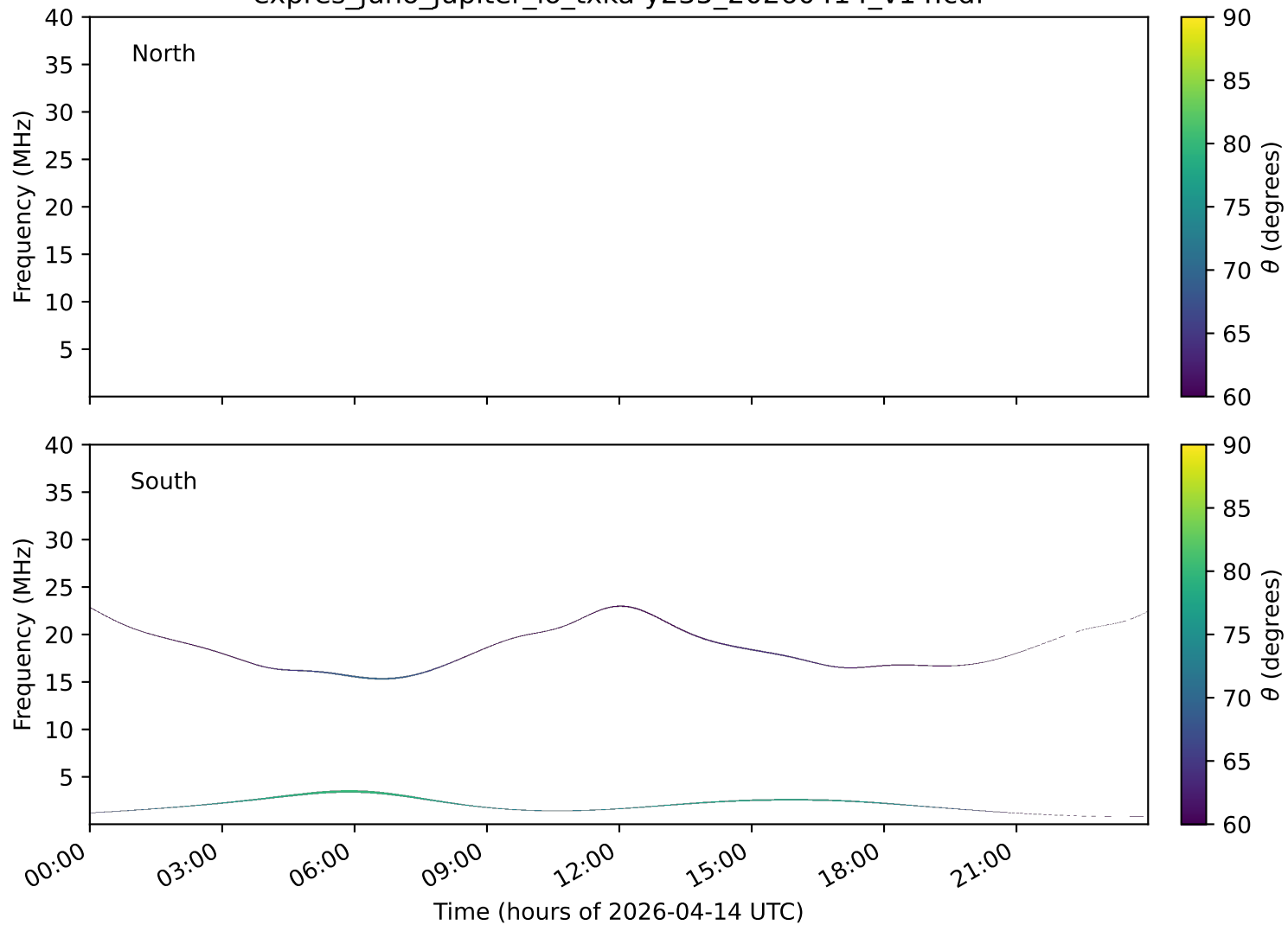
expres_juno_jupiter_io_txka-y235_20260414_v14.cdf
