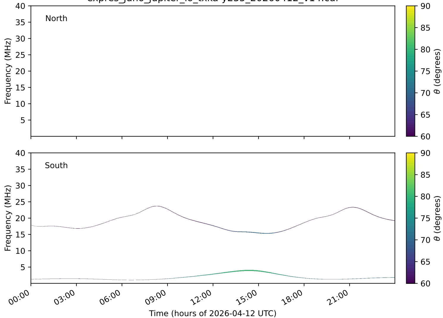
expres_juno_jupiter_io_txka-y235_20260412_v14.cdf
