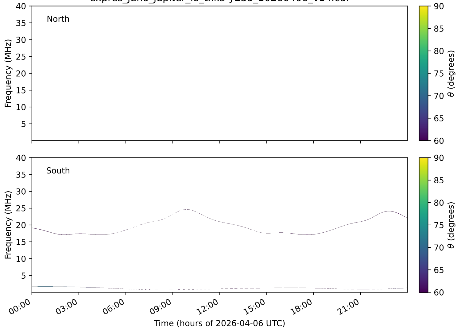
expres_juno_jupiter_io_txka-y235_20260406_v14.cdf
