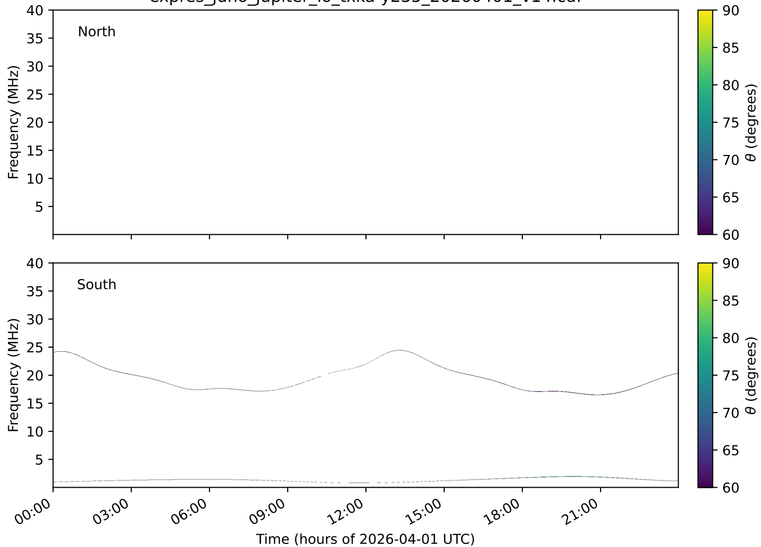
expres_juno_jupiter_io_txka-y235_20260401_v14.cdf
