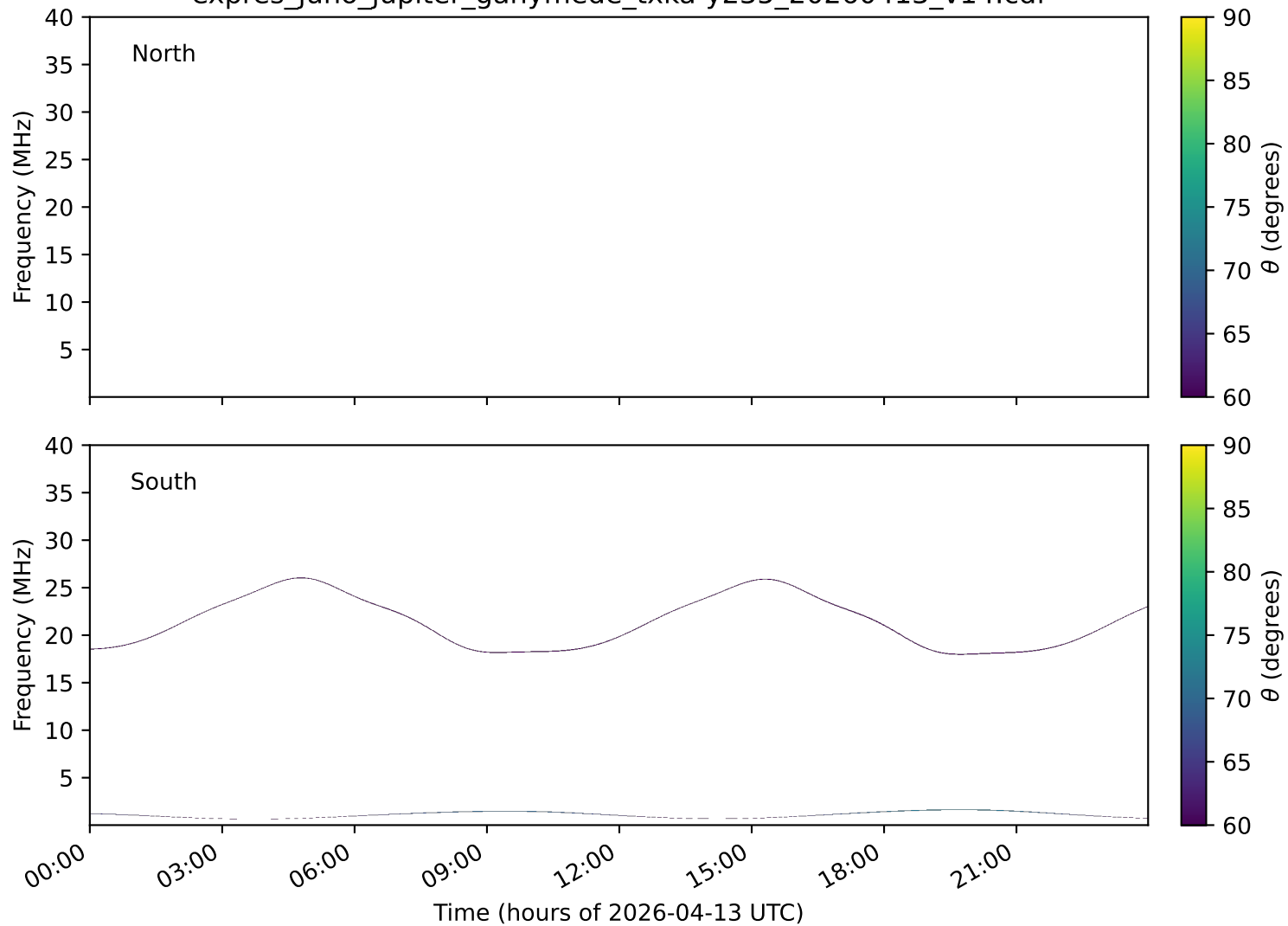
expres_juno_jupiter_ganymede_txka-y235_20260413_v14.cdf
