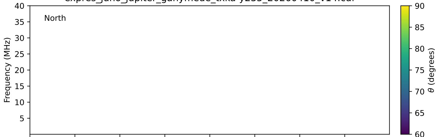
expres_juno_jupiter_ganymede_txka-y235_20260410_v14.cdf
