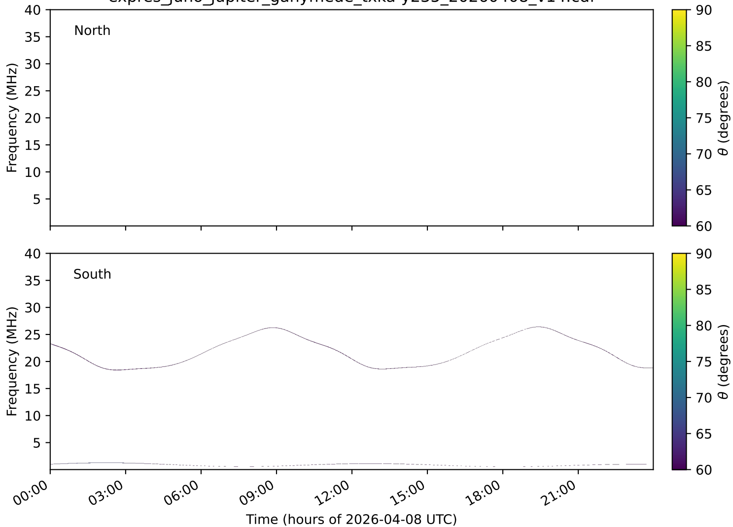
expres_juno_jupiter_ganymede_txka-y235_20260408_v14.cdf
