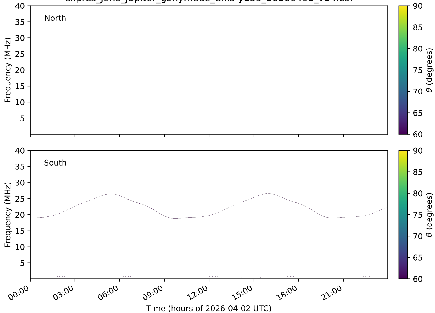
expres_juno_jupiter_ganymede_txka-y235_20260402_v14.cdf
