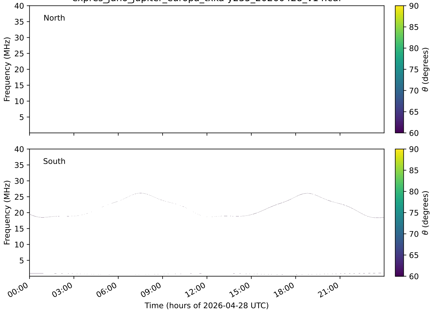
expres_juno_jupiter_europa_txka-y235_20260428_v14.cdf
