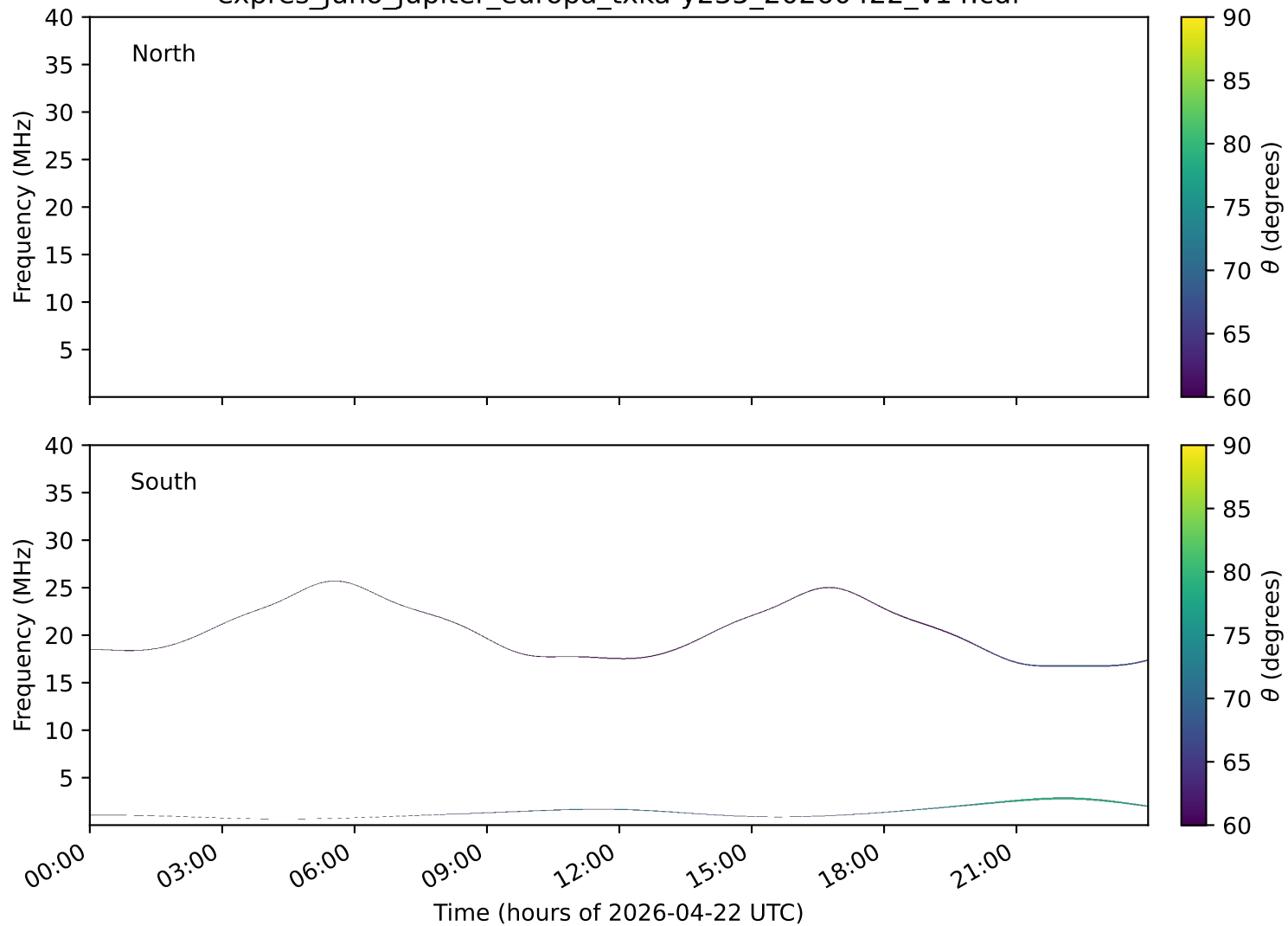
expres_juno_jupiter_europa_txka-y235_20260422_v14.cdf
