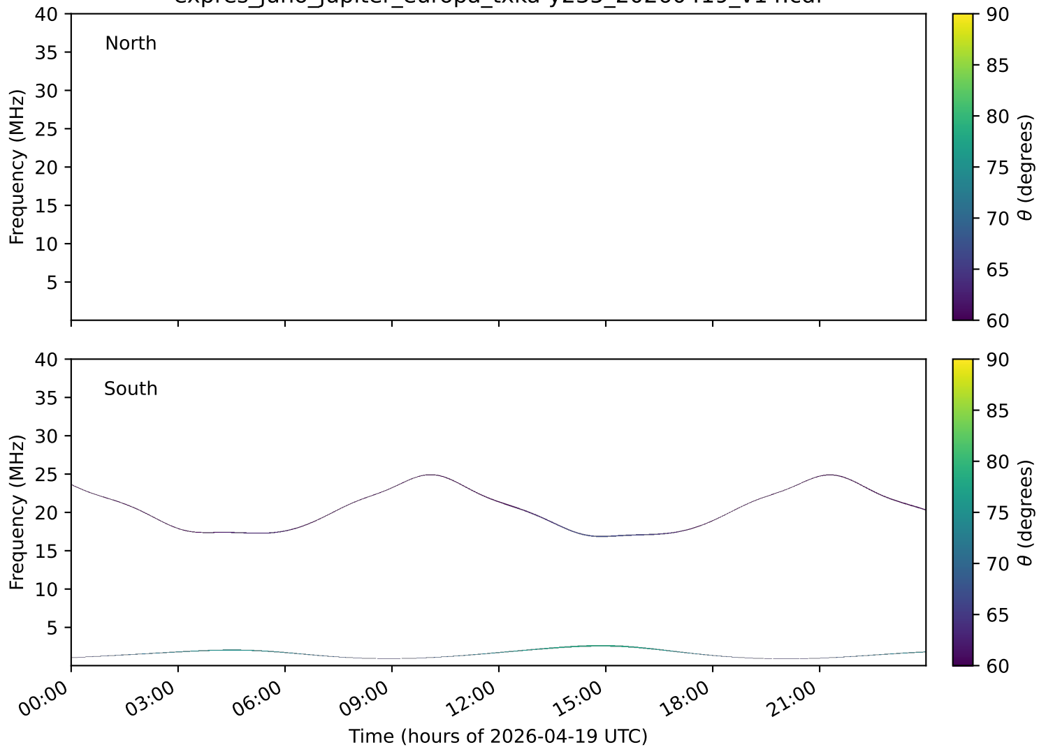
expres_juno_jupiter_europa_txka-y235_20260419_v14.cdf
