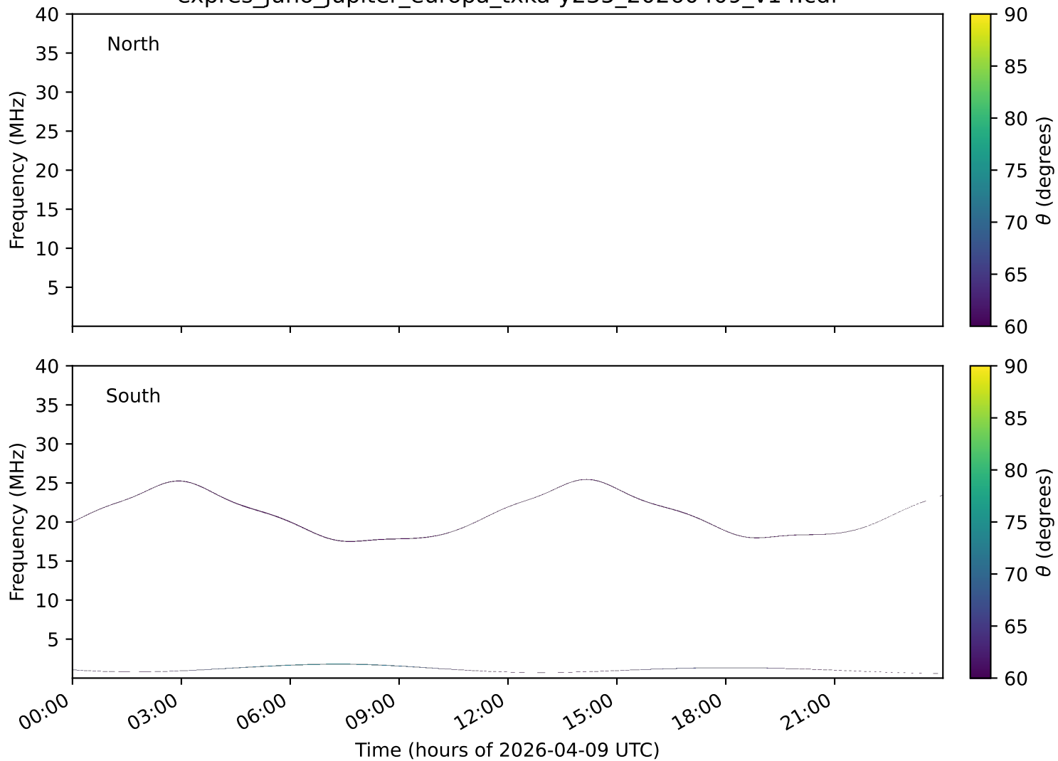
expres_juno_jupiter_europa_txka-y235_20260409_v14.cdf
