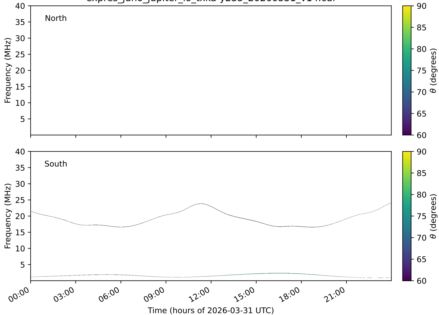
expres_juno_jupiter_io_txka-y235_20260331_v14.cdf
