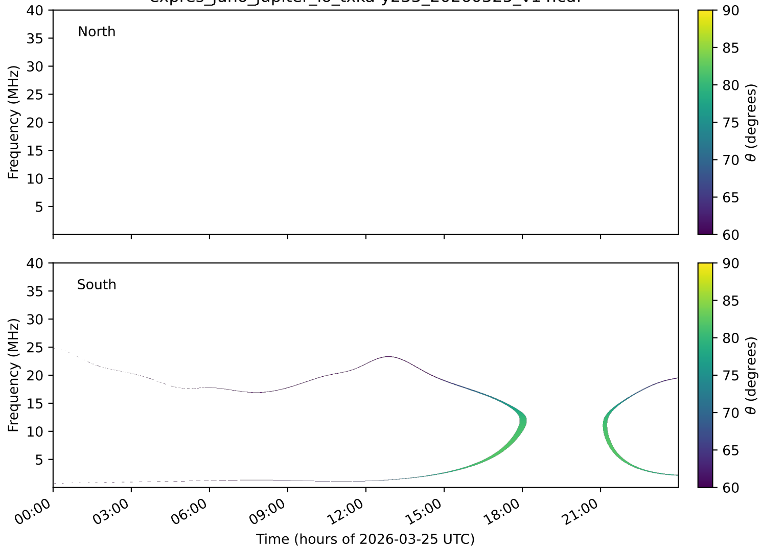
expres_juno_jupiter_io_txka-y235_20260325_v14.cdf
