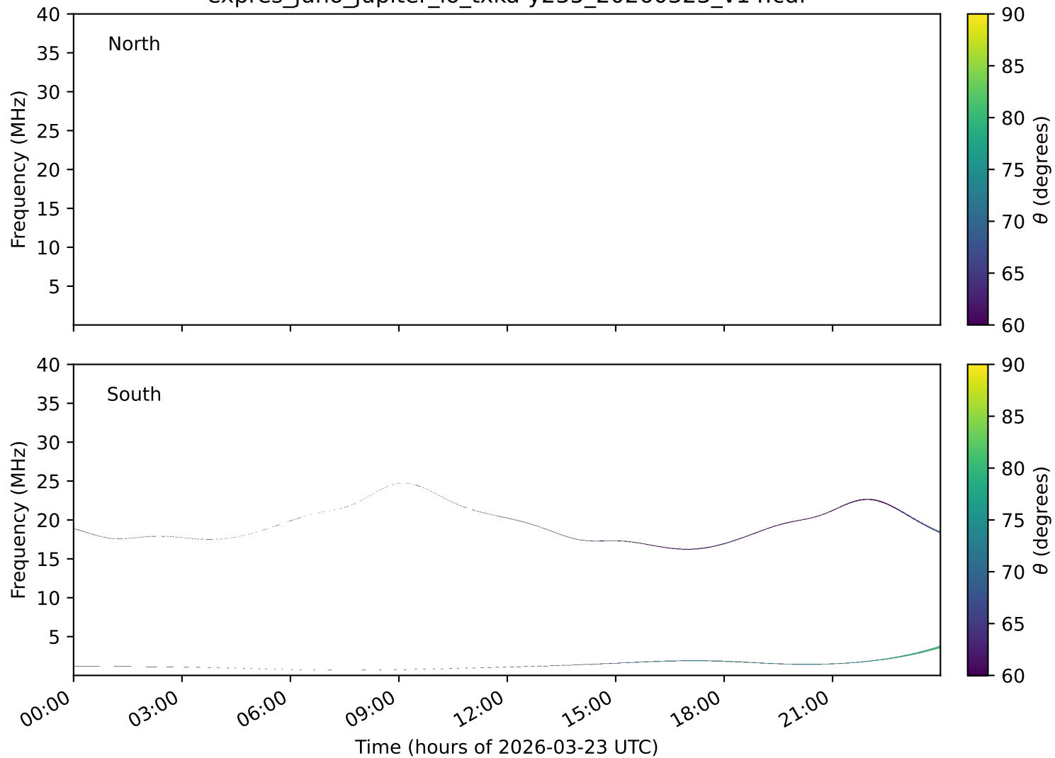
expres_juno_jupiter_io_txka-y235_20260323_v14.cdf
