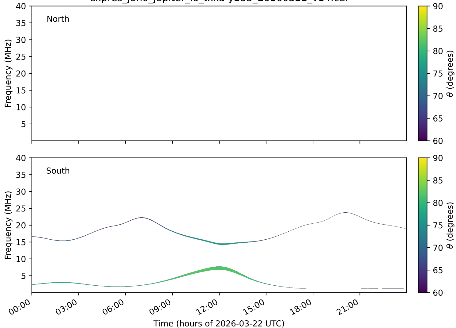
expres_juno_jupiter_io_txka-y235_20260322_v14.cdf
