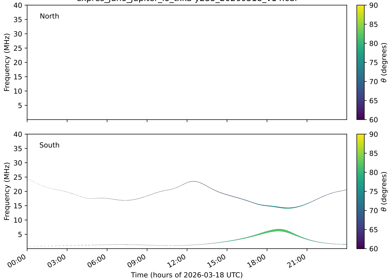
expres_juno_jupiter_io_txka-y235_20260318_v14.cdf
