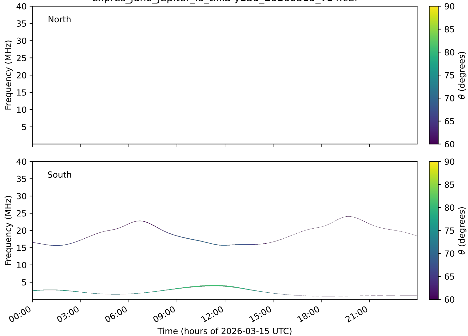
expres_juno_jupiter_io_txka-y235_20260315_v14.cdf
