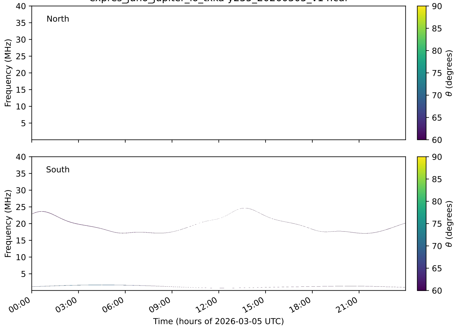
expres_juno_jupiter_io_txka-y235_20260305_v14.cdf
