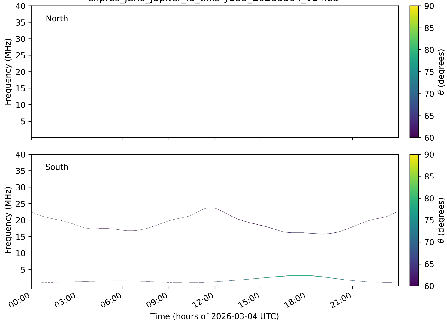
expres_juno_jupiter_io_txka-y235_20260304_v14.cdf
