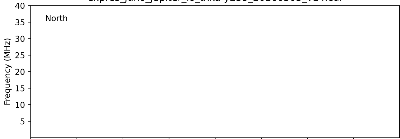
expres_juno_jupiter_io_txka-y235_20260303_v14.cdf
