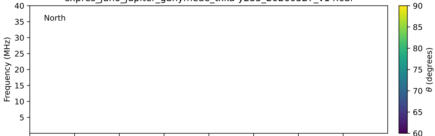
expres_juno_jupiter_ganymede_txka-y235_20260327_v14.cdf
