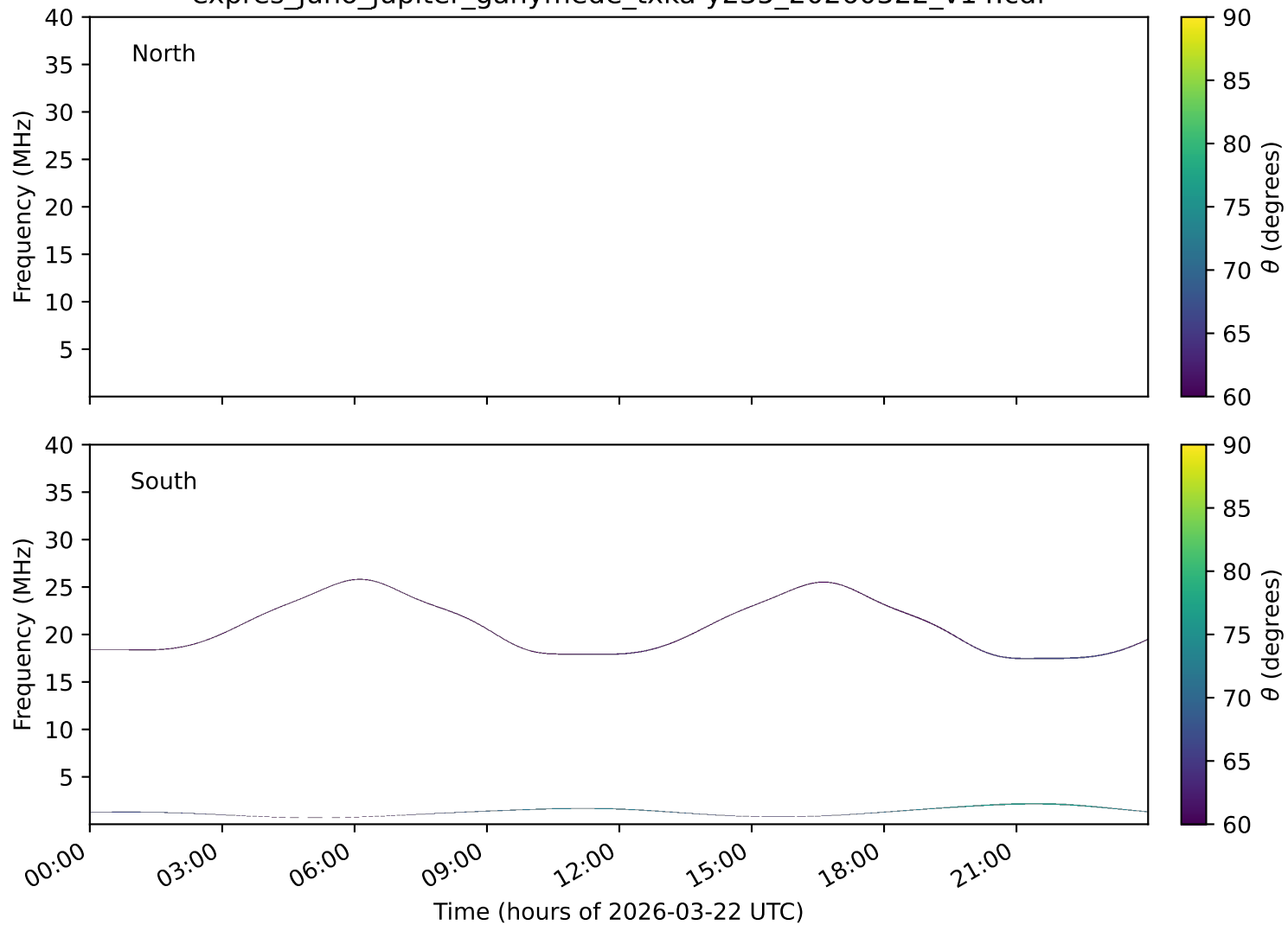
expres_juno_jupiter_ganymede_txka-y235_20260322_v14.cdf
