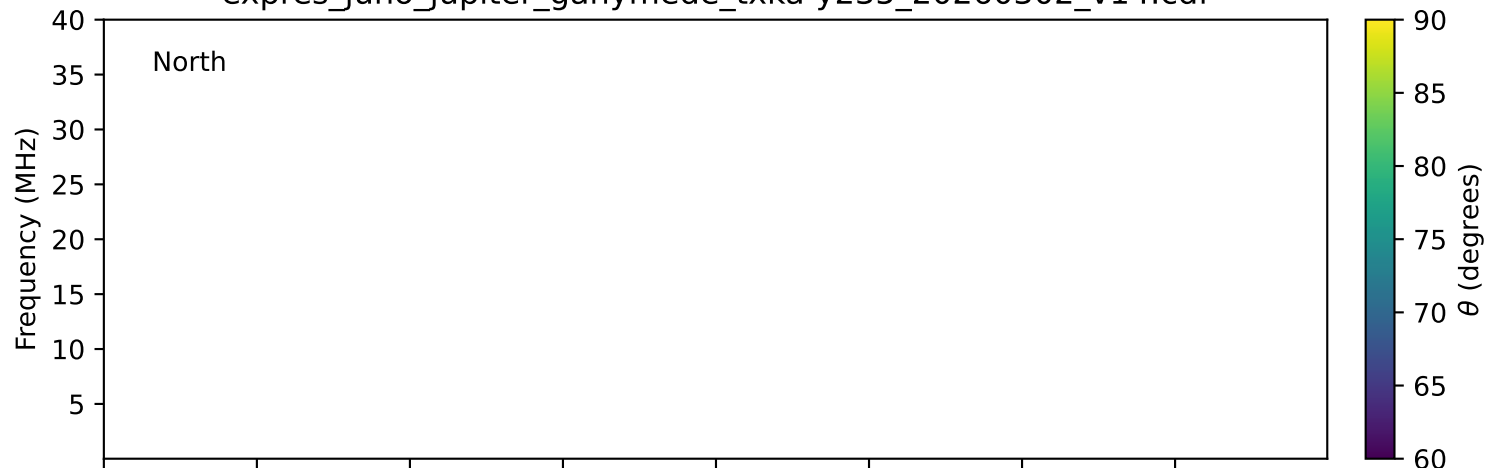
expres_juno_jupiter_ganymede_txka-y235_20260302_v14.cdf
