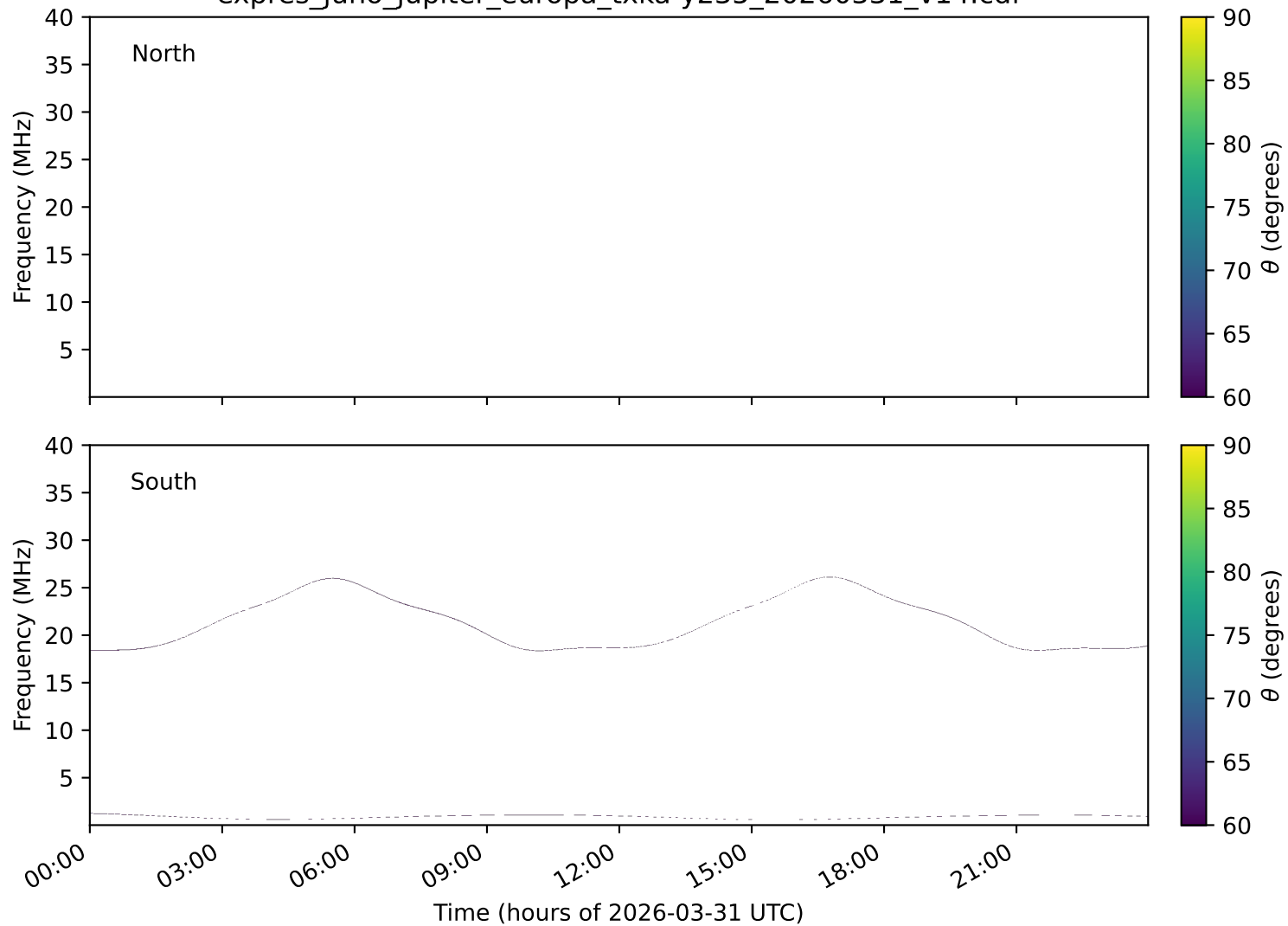
expres_juno_jupiter_europa_txka-y235_20260331_v14.cdf
