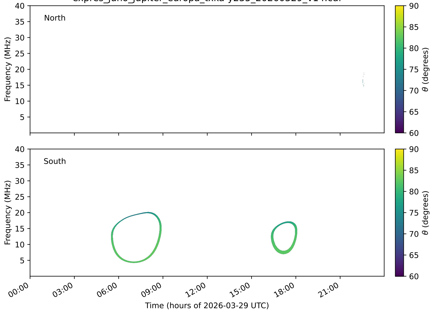
expres_juno_jupiter_europa_txka-y235_20260329_v14.cdf
