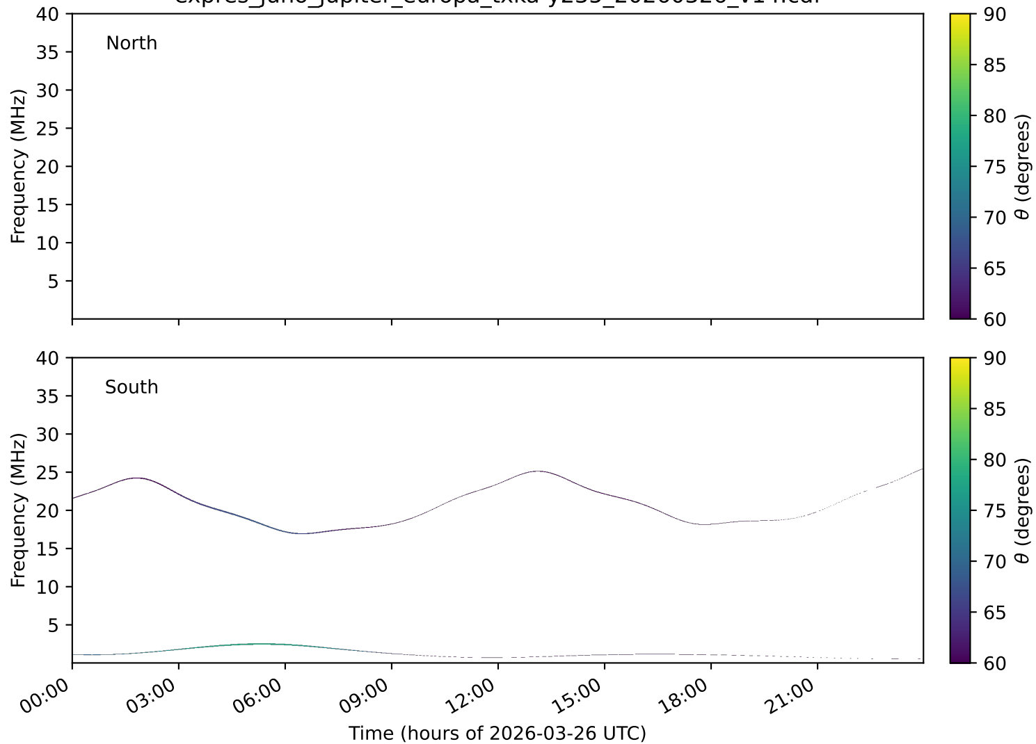
expres_juno_jupiter_europa_txka-y235_20260326_v14.cdf
