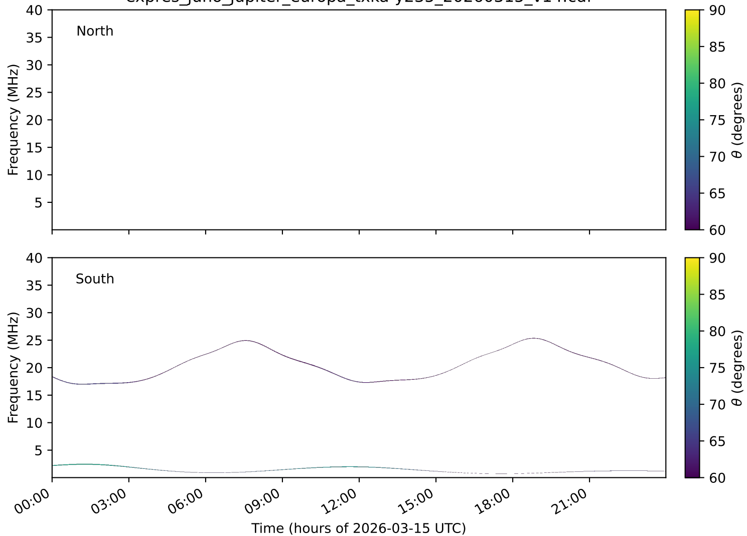
expres_juno_jupiter_europa_txka-y235_20260315_v14.cdf
